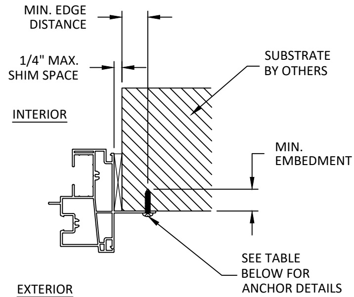
C 7 HORIZONTAL SECTION JAMB INSTALLATION
