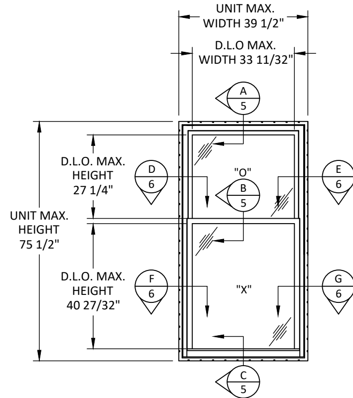
TYPICAL ELEVATION SINGLE HUNG WINDOW (COTTAGE) DP50
