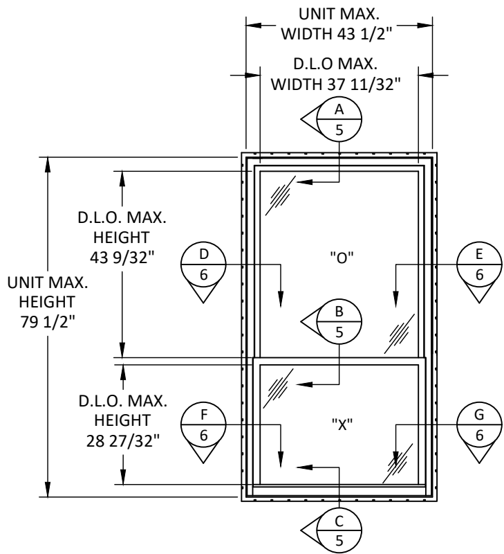
TYPICAL ELEVATION SINGLE HUNG WINDOW (ORIEL) DP35
