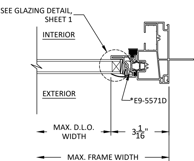
E 6 HORIZONTAL SECTION FIXED RIGHT JAMB
