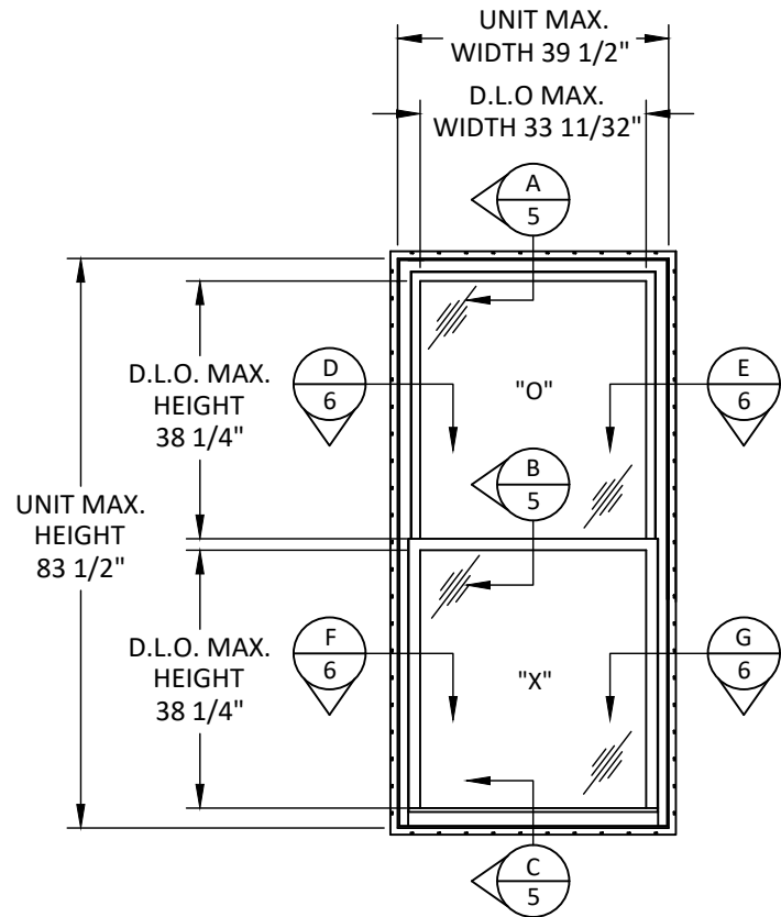
TYPICAL ELEVATION SINGLE HUNG WINDOW (EQUAL) DP35
