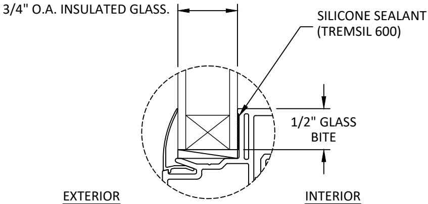
GLAZING DETAIL 1
