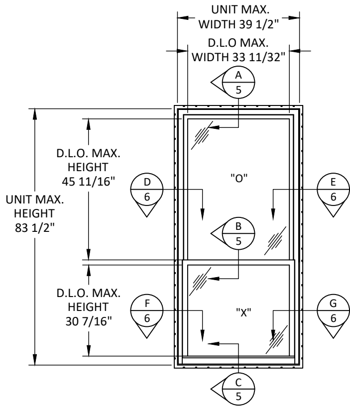
TYPICAL ELEVATION SINGLE HUNG WINDOW (ORIEL) DP35
