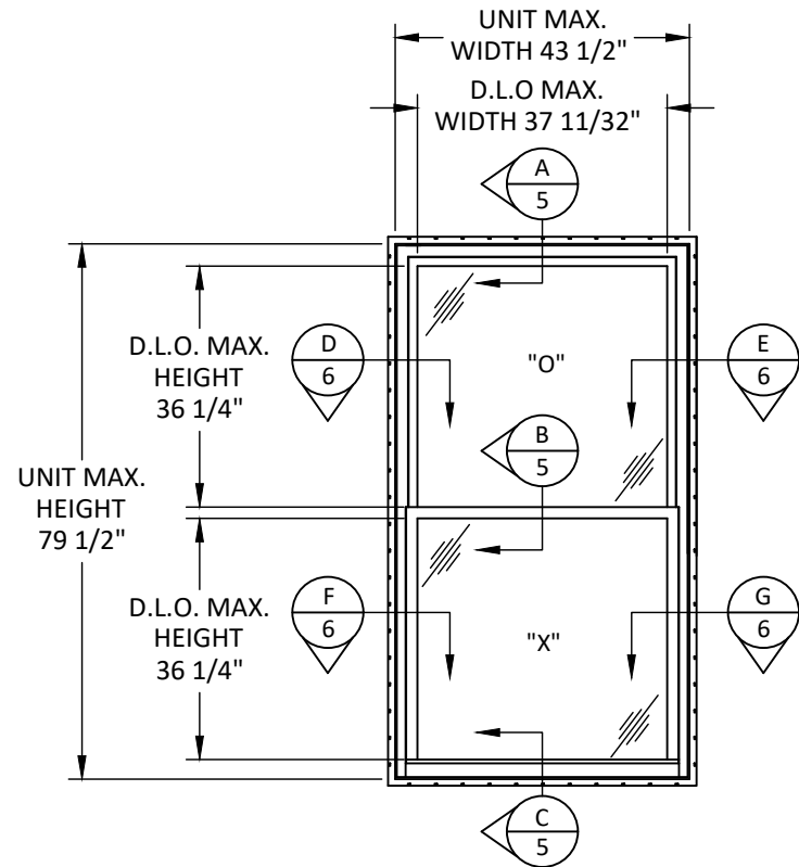
TYPICAL ELEVATION SINGLE HUNG WINDOW (EQUAL) DP35
