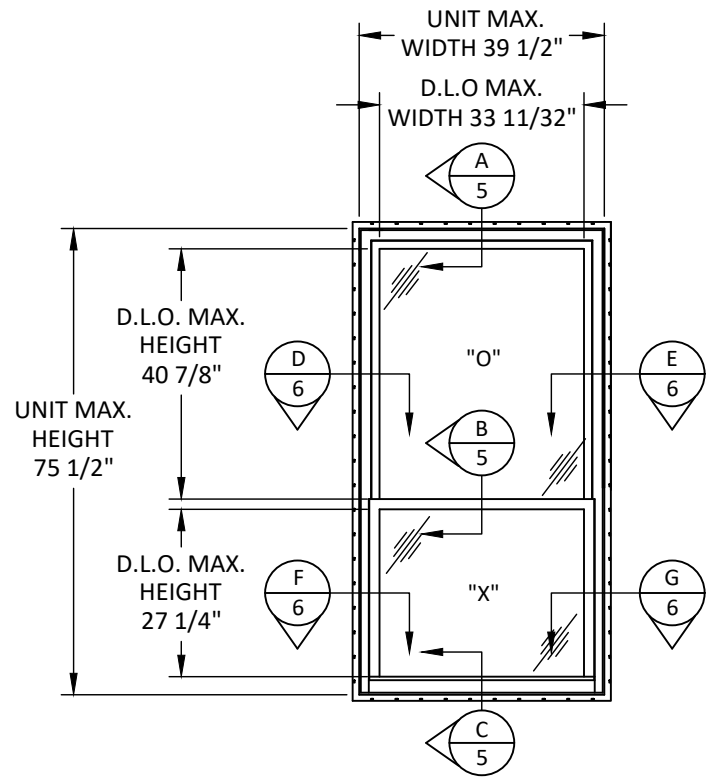
TYPICAL ELEVATION SINGLE HUNG WINDOW (ORIEL) DP50
