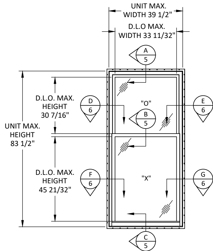
TYPICAL ELEVATION SINGLE HUNG WINDOW (COTTAGE) DP35
