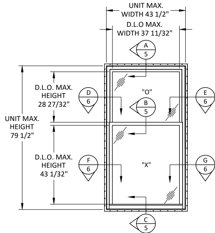
TYPICAL ELEVATION SINGLE HUNG WINDOW (COTTAGE) DP35
