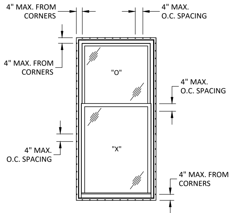
ANCHOR LAYOUT NAILING FIN
