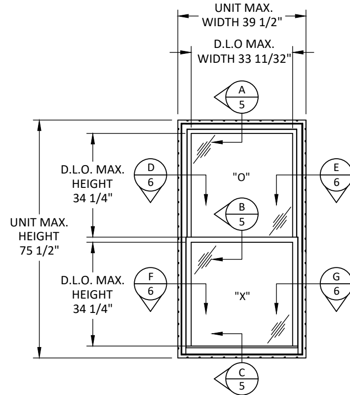
TYPICAL ELEVATION SINGLE HUNG WINDOW (EQUAL) DP50
