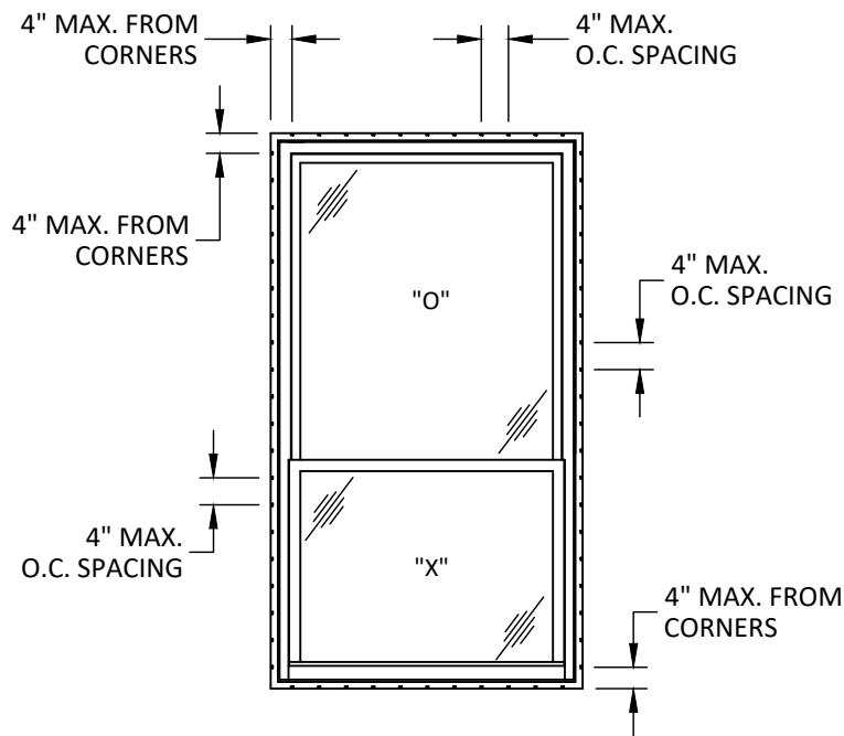
ANCHOR LAYOUT NAILING FIN
